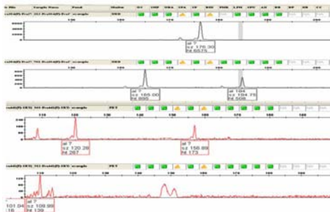
Micro-satellite genotypes of some of the scat samples after fragment analysis with Genemapper software
